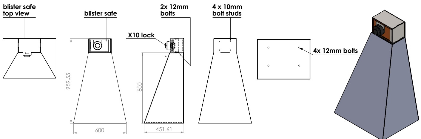
MODEL GKC1-S - FRONT
